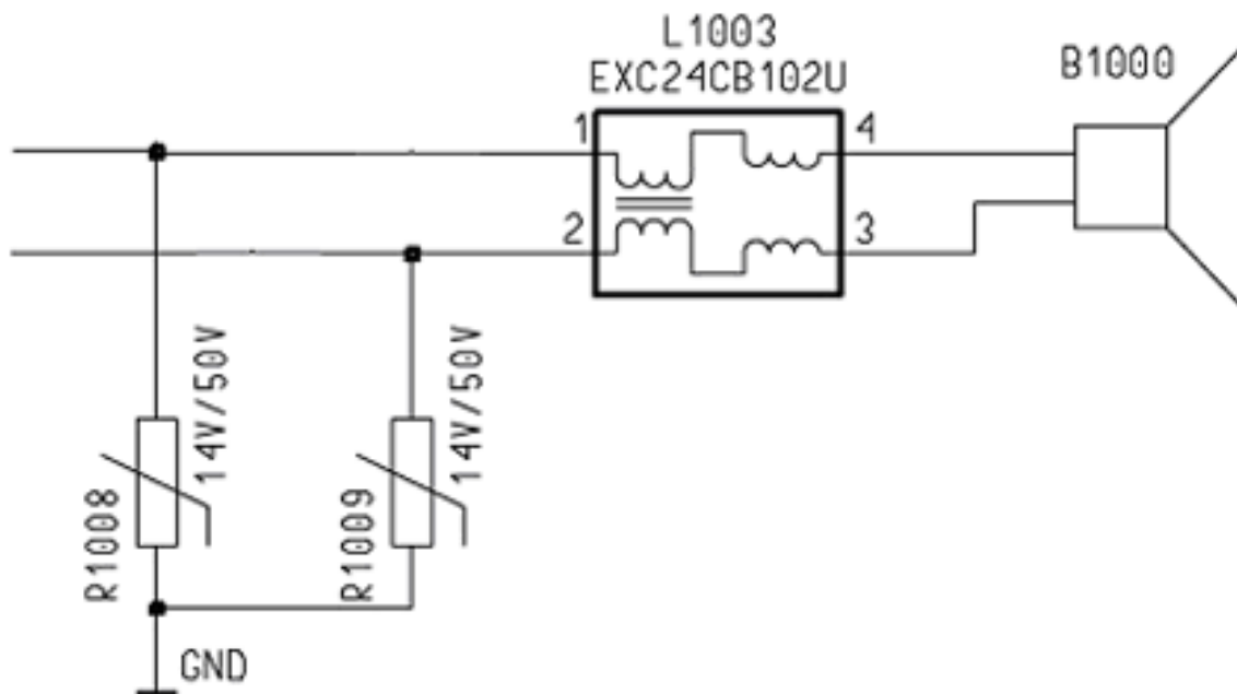
Figure 114 Internal earpiece circuitry
