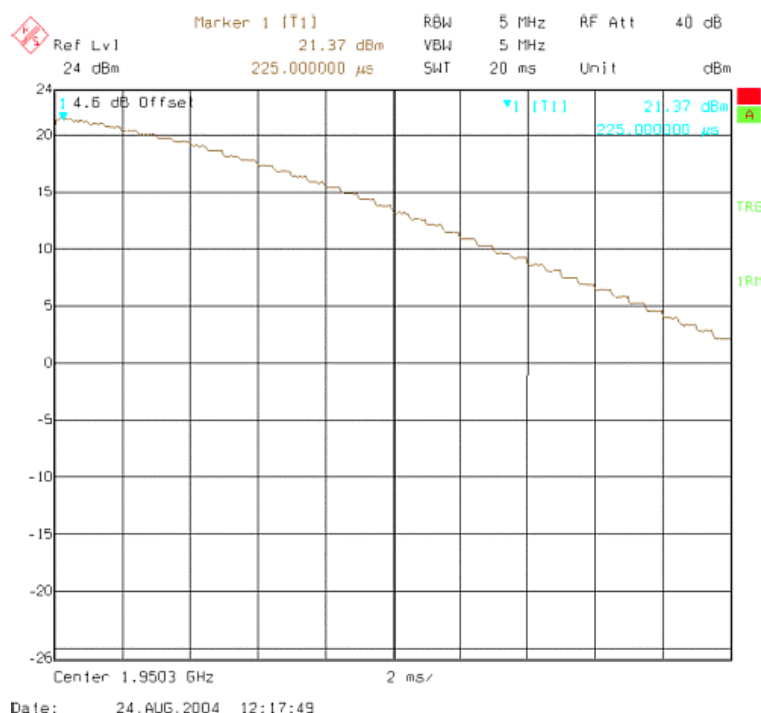
Figure 70 High burst measurement
