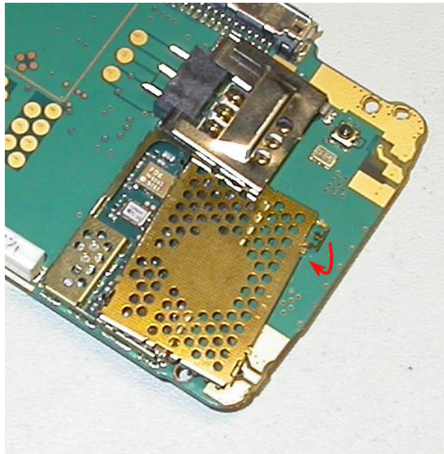
Figure 77 Bending the lock pin and the area around it
