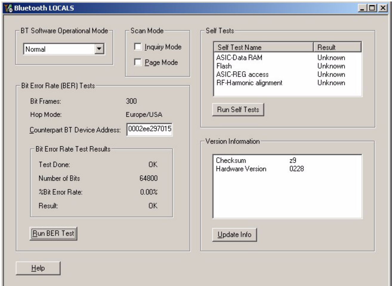
Figure 51 Phoenix settings for Bluetooth troubleshooting
