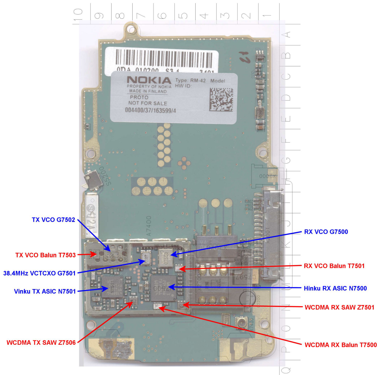
Figure 56 RF key component placement, bottom
