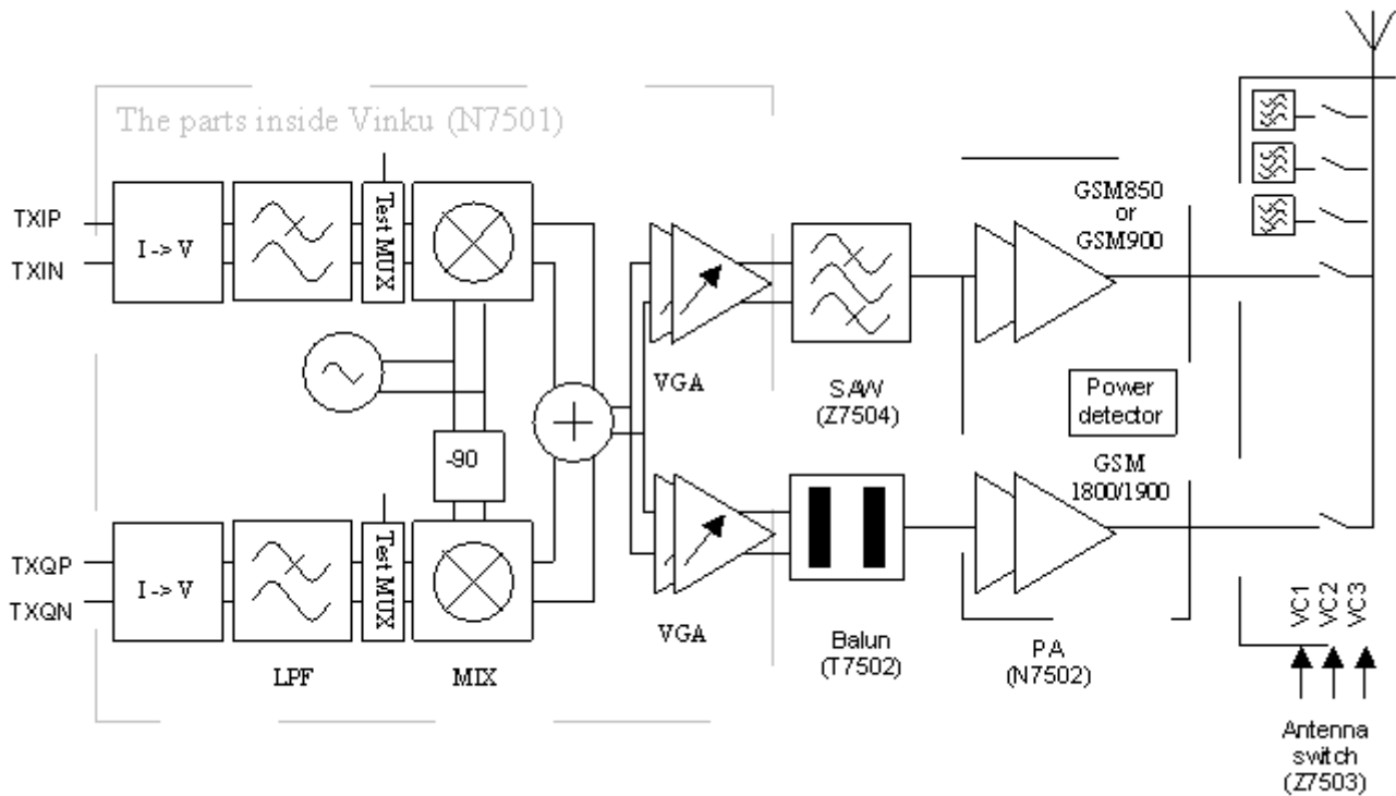
Figure 125 GSM transmitter
