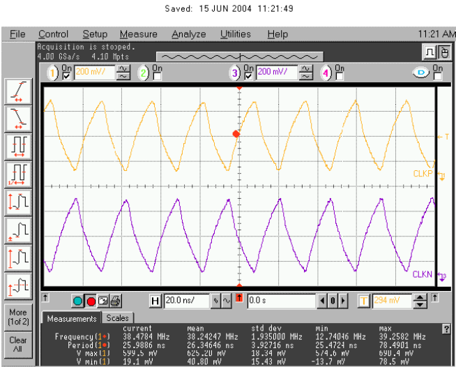
Figure 43 SYSCLK from J2801
