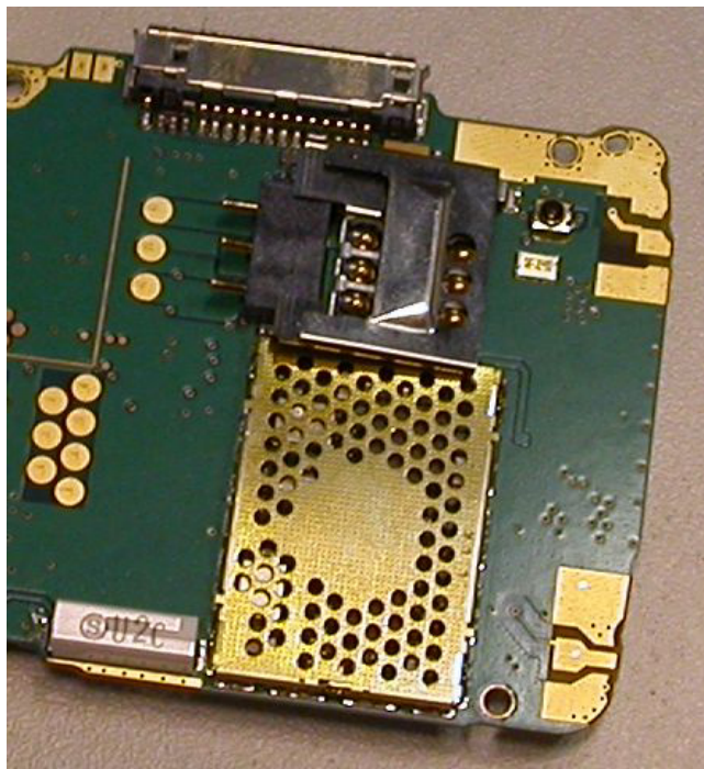
Figure 78 The shield lid in place
