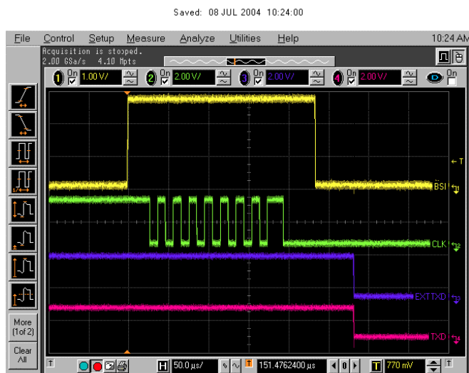
Figure 45 Flashing pic 1. Take single trig measurement for the rise of the BSI signal.
