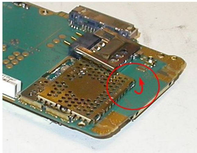
Figure 72 Bending the lock pin and the area around it
