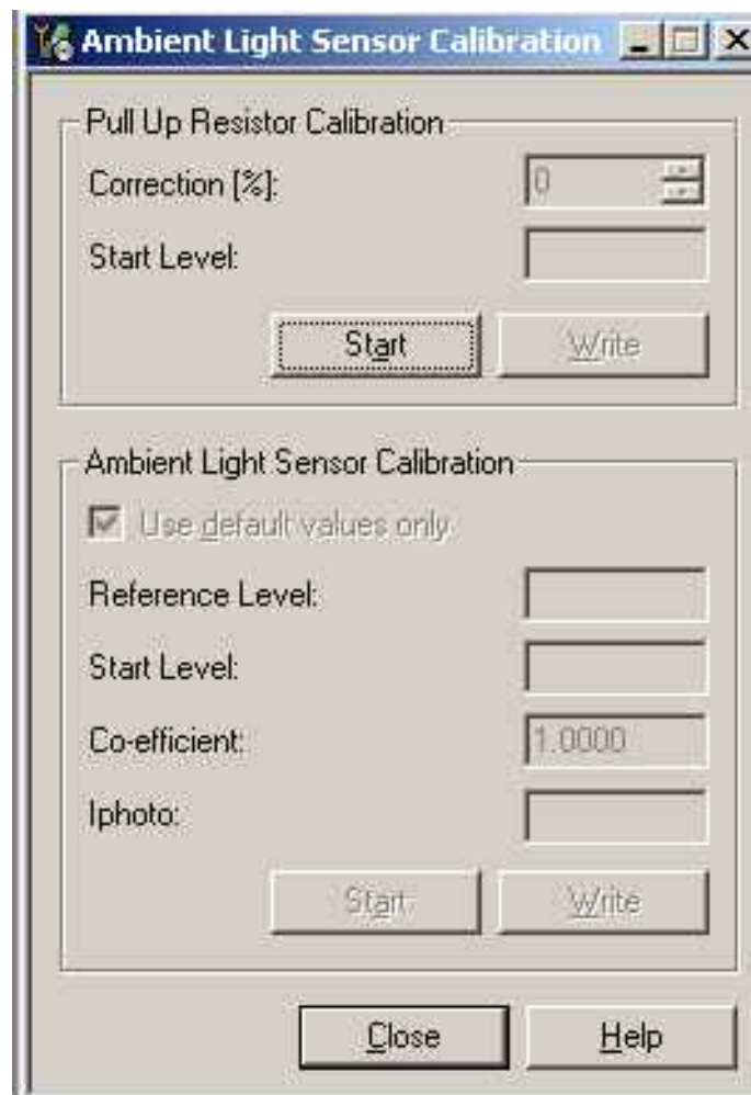
Figure 50 Ambient Light Sensor Calibration window
