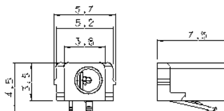
Figure 118 Charger connector
