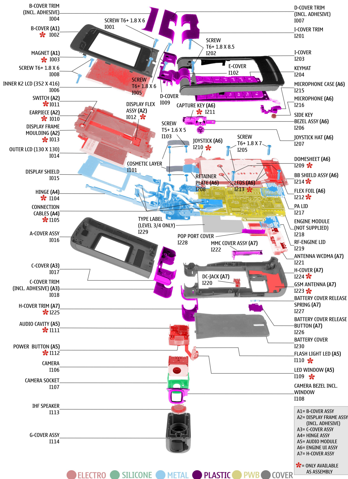
Figure 2 RM-42 exploded view
