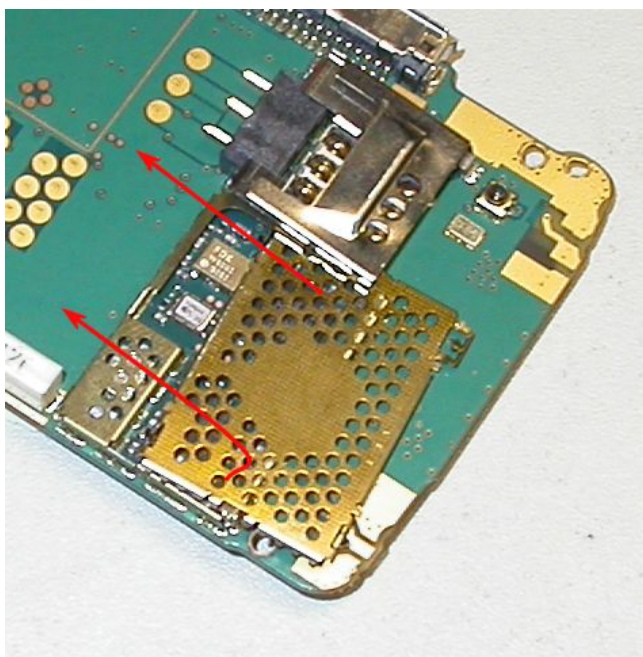
Figure 73 Sliding the shield lid
