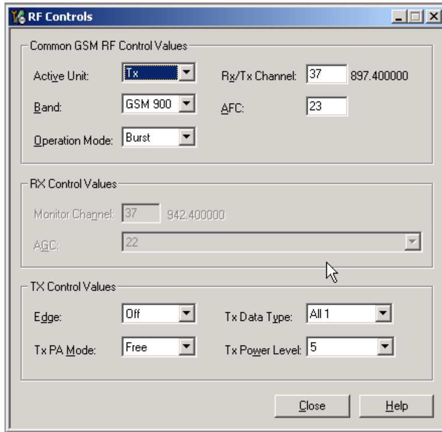
Figure 65 RF Controls window
