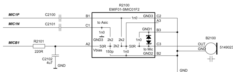
Figure 112 Internal microphone circuitry
