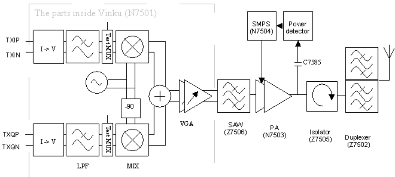
Figure 123 WCDMA transmitter
