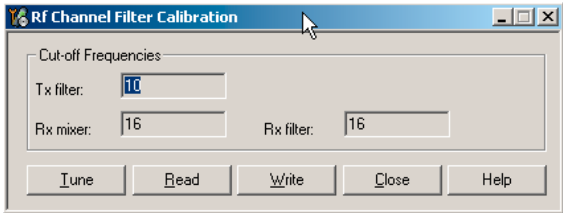
Figure 69 RF channel filter calibration typical values
