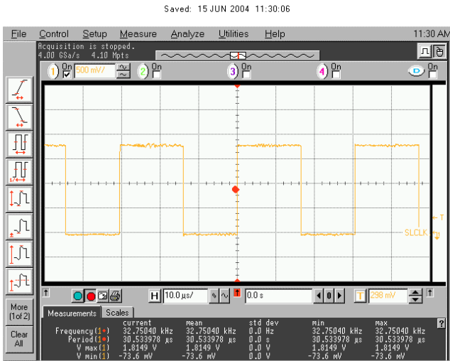
Figure 44 SleepCLK from R211
