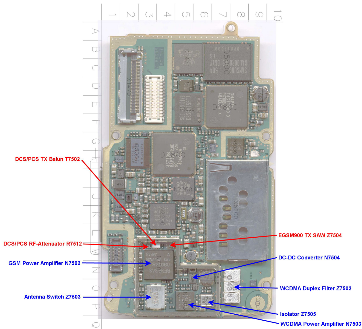
Figure 57 RF key component placement, top
