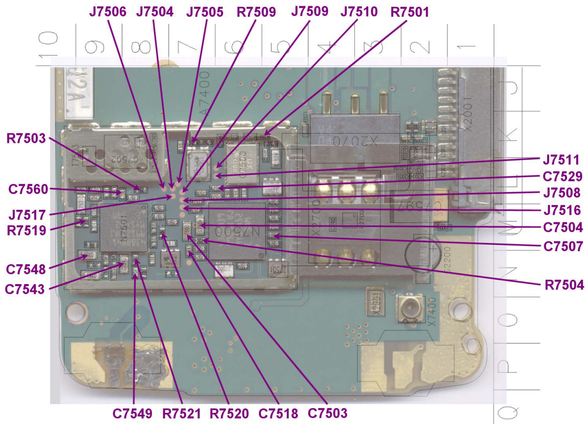
Figure 60 Test points for oscilloscope, bottom
