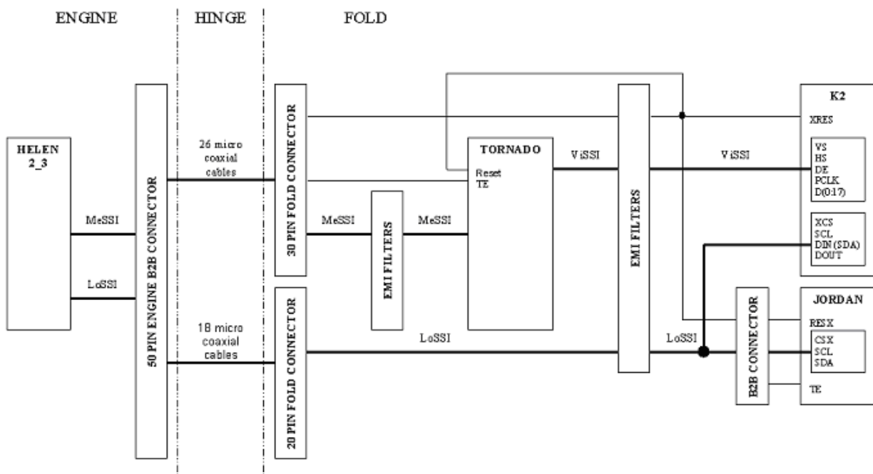
Figure 108 LoSSI signals in RM-42
