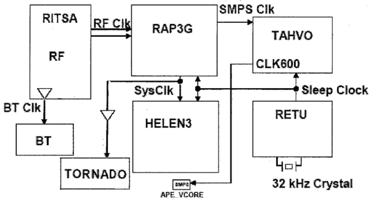
Figure 102 Clocking scheme
