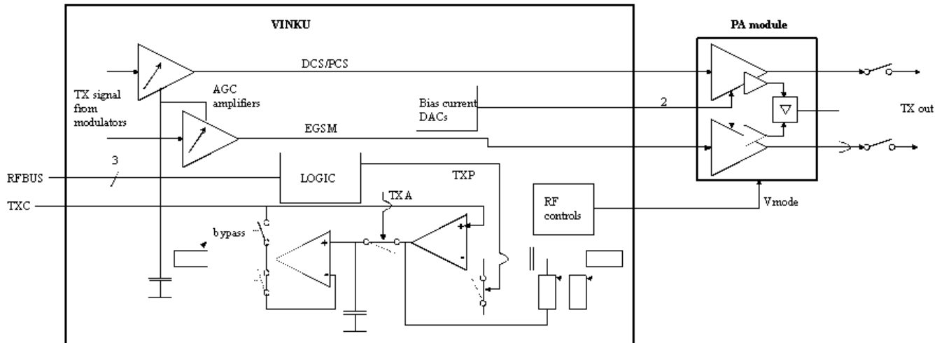
Figure 126 GSM/EDGE power control topology and control signals
