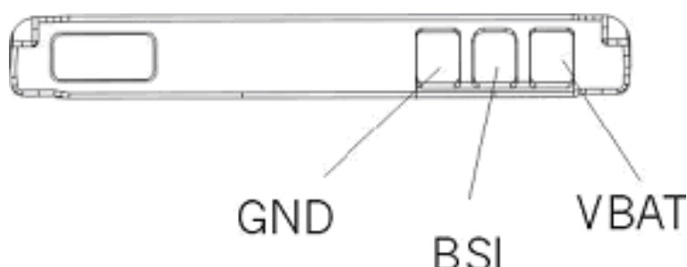
Figure 119 Battery connector
