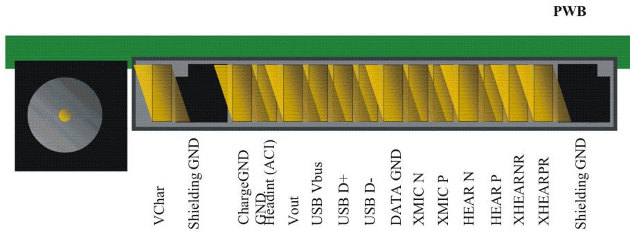
Figure 117 External audio connector
