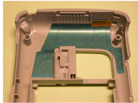
Figure 68 GSM antenna radiator
