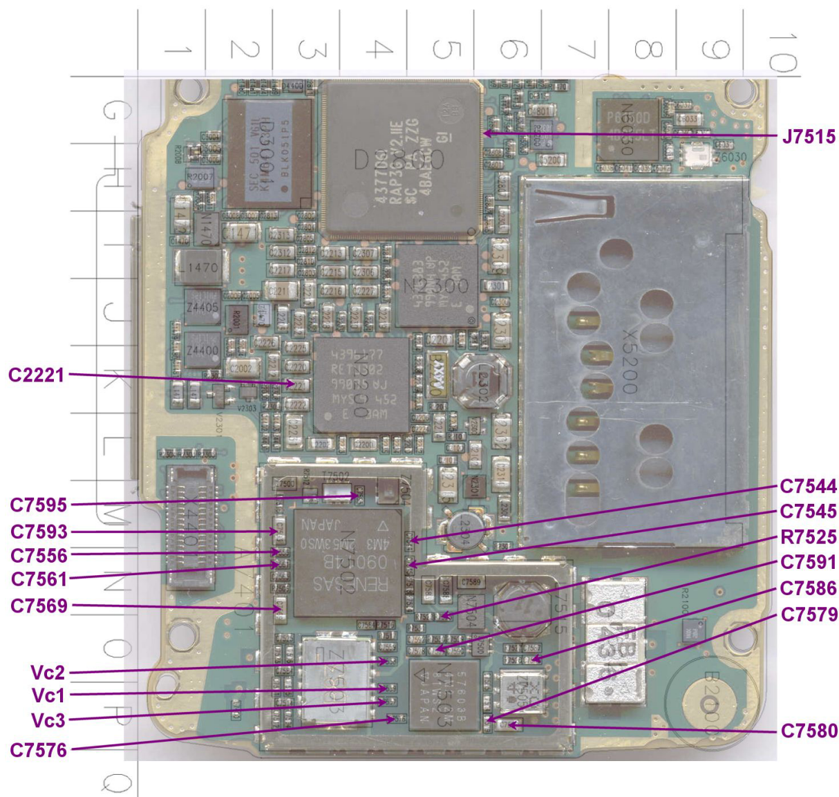
Figure 61 Test points for oscilloscope, top
