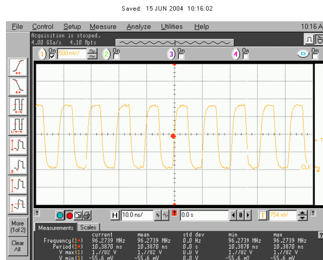
Figure 47 CMT SDRAM CLK from pin J2804
