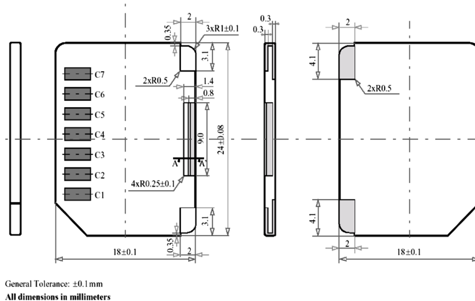
Figure 103 Reduced size MMC
