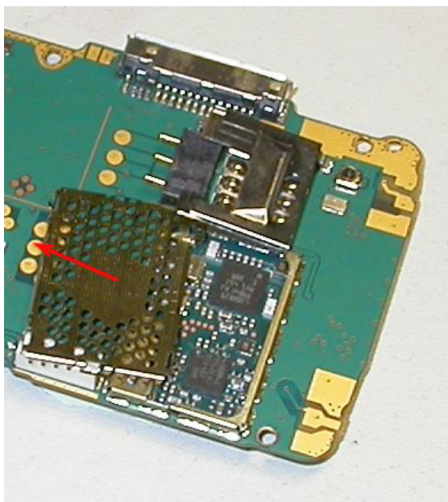
Figure 74 Removing the shield lid
