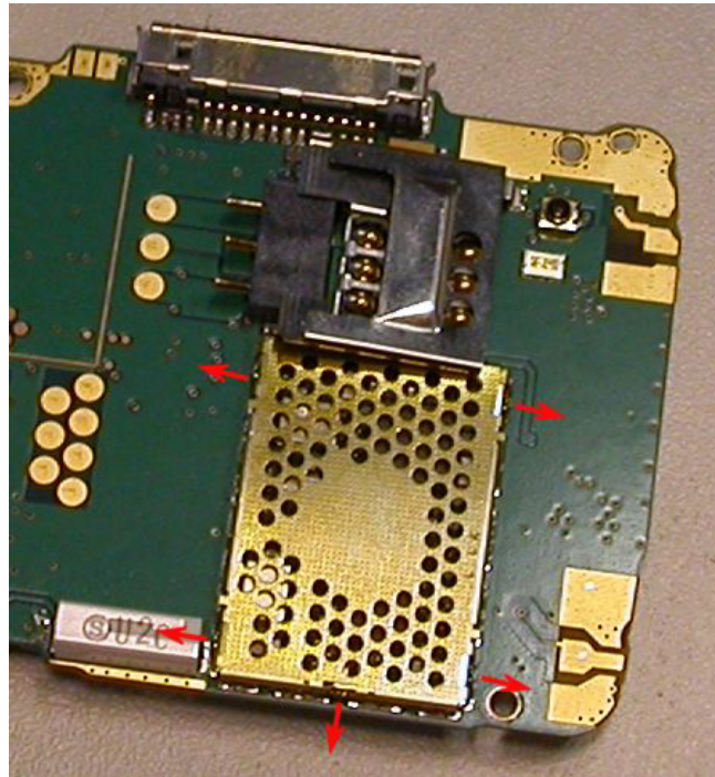
Figure 71 Opening the lock pins
