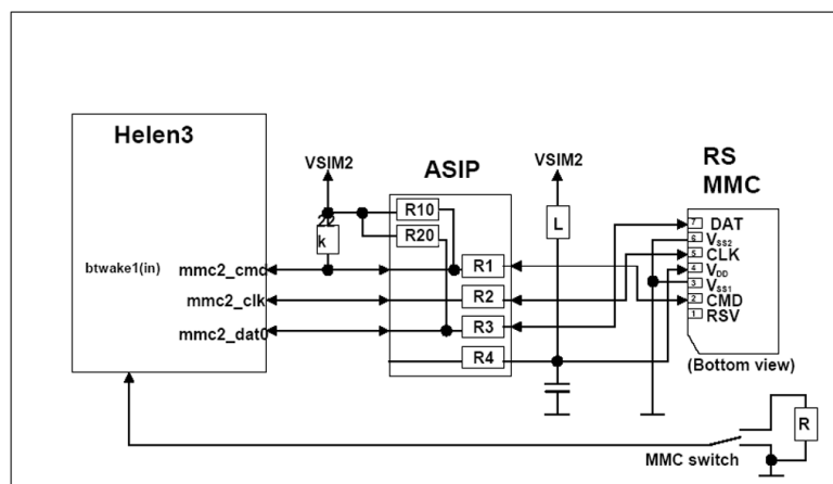
Figure 104 MMC interface
