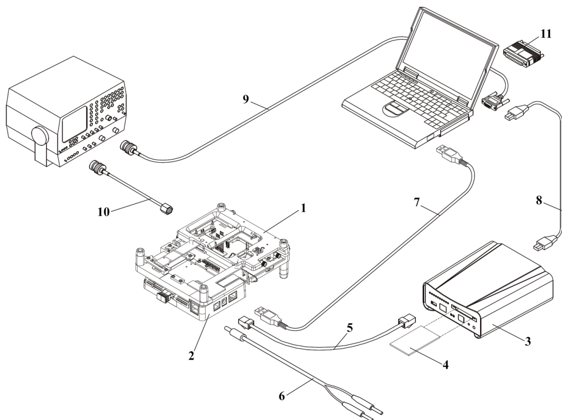
Figure 36 MJ-48 module jig service concept
