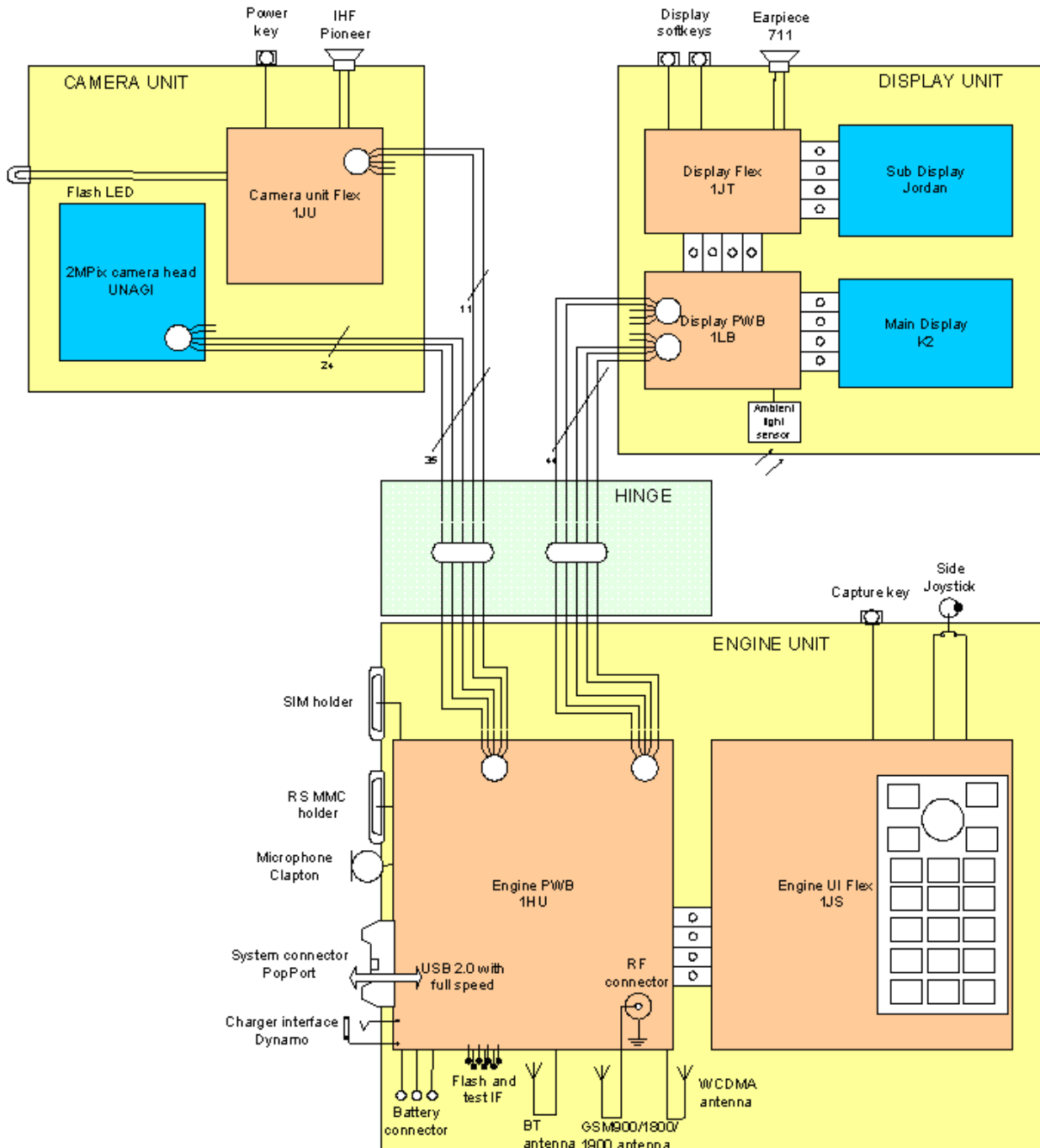
Figure 96 Internal and external connections diagram
