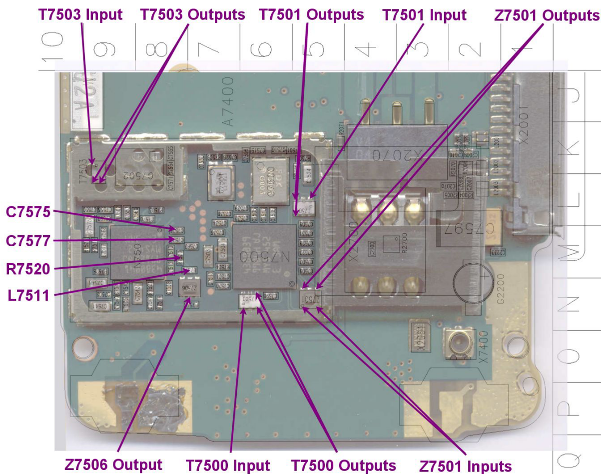
Figure 58 Test point locations for spectrum analyzer, bottom
