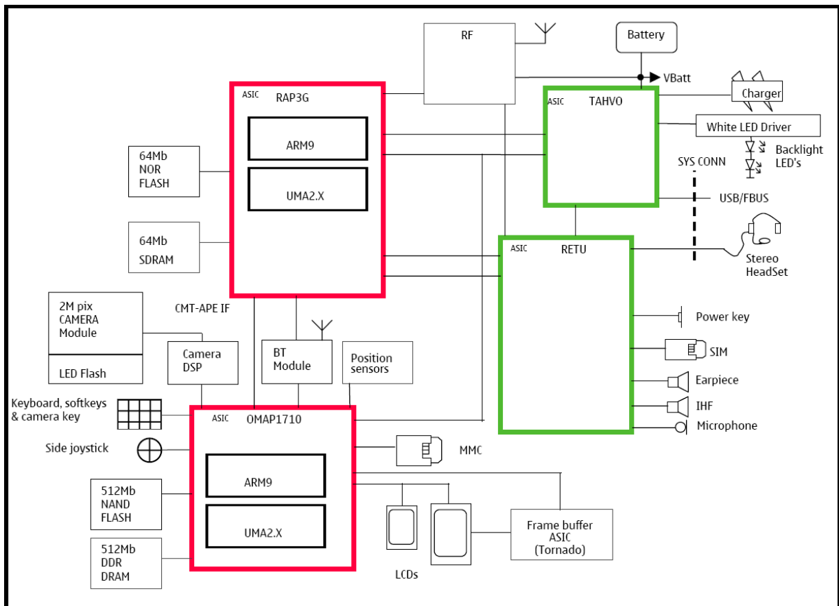
Figure 97 Functional block diagram
