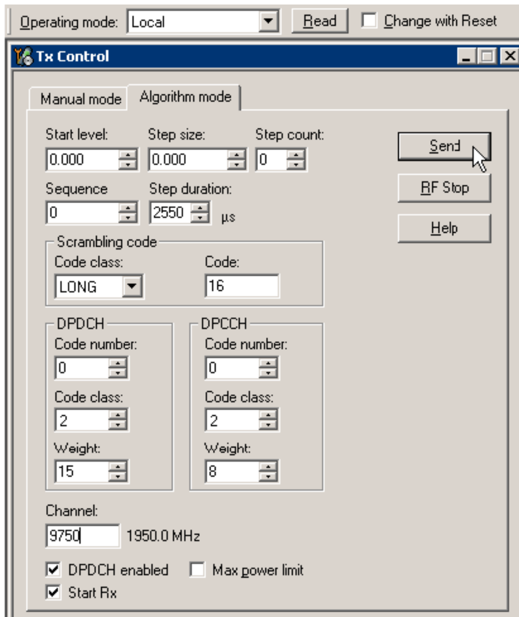
Figure 66 Tx Control window
