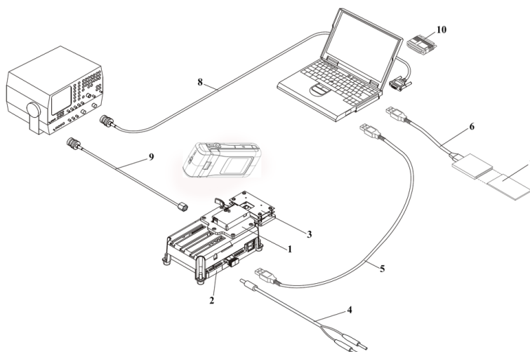
Figure 40 RF testing concept with RF coupler
