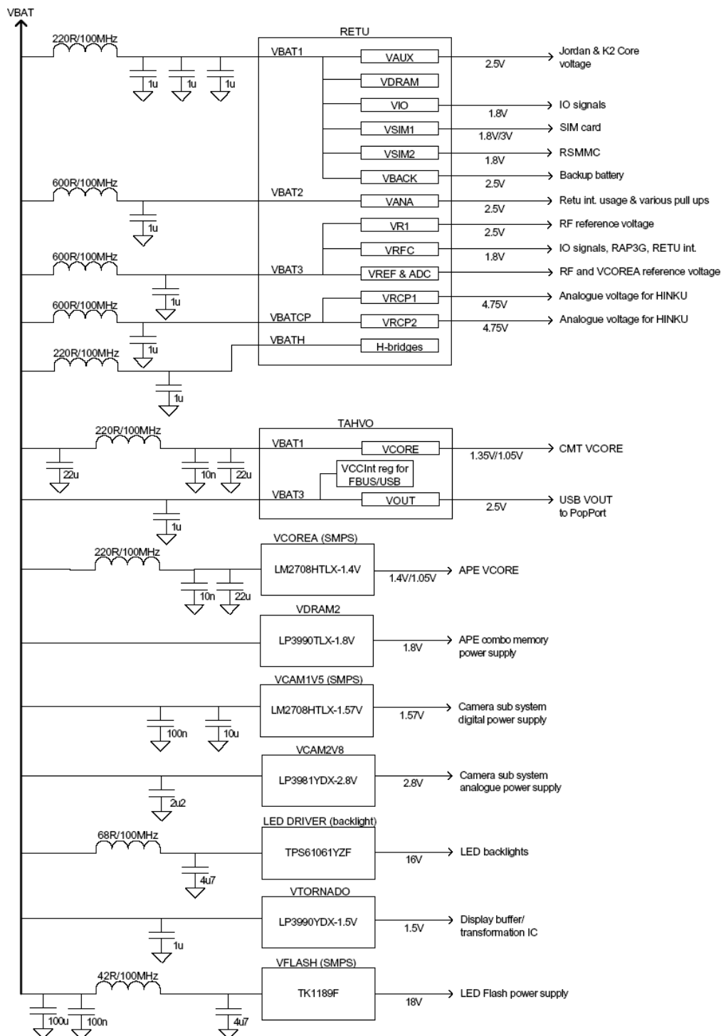
Figure 100 Power distribution diagram
