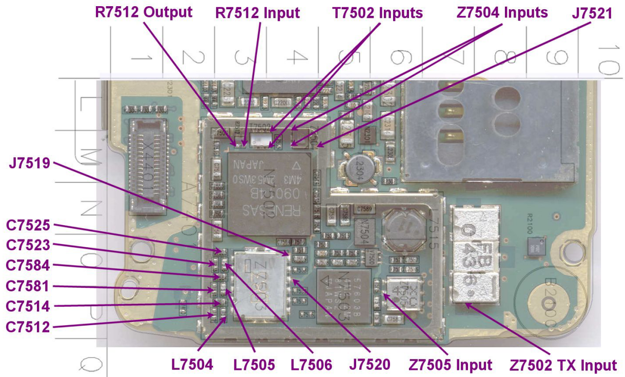
Figure 59 Test point locations for spectrum analyzer, top
